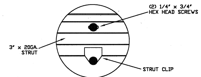
TYPICAL TOP STRUT ATTACHMENT N.T.S. ③
