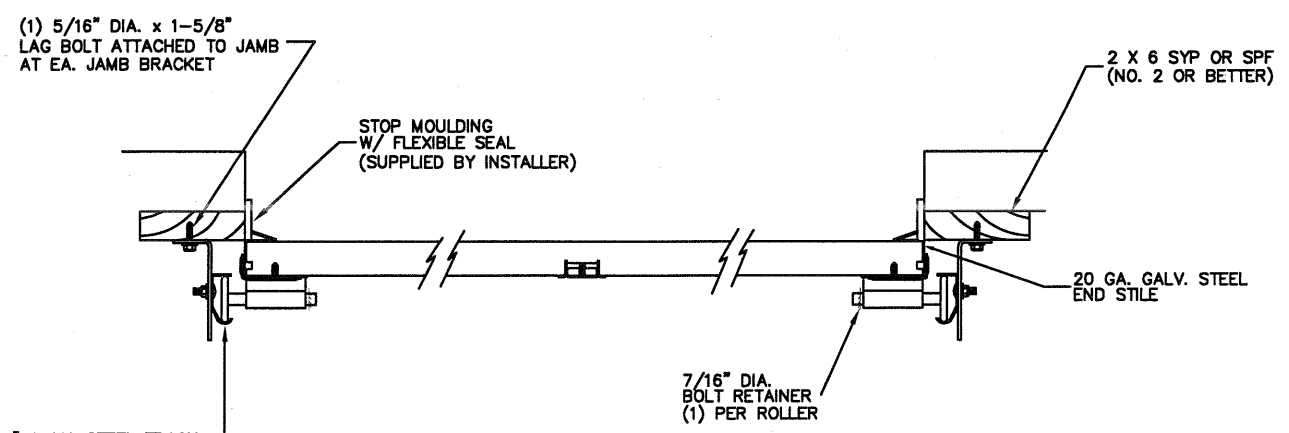
TRACK MOUNTING DETAIL N.T.S.
